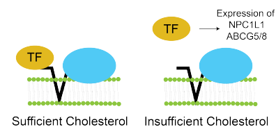
Figure 45: Regulation of SREBP2. When there is insufficient cholesterol, SREBP2 is cleaved releasing the transcription factor (TF) fragment, where it can go to the nucleus and drive expression of cholesterol uptake genes such as NPC1L1, ABCG5/8. This means that at sufficient cholesterol levels absorption is largely reduced.
