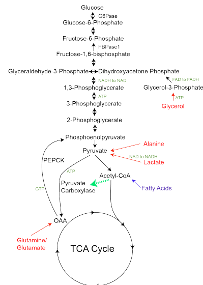
Figure 36: Schematic of gluconeogenesis. Red indicates key gluconeogenic substrates while green indicates energy consuming or generating steps.
